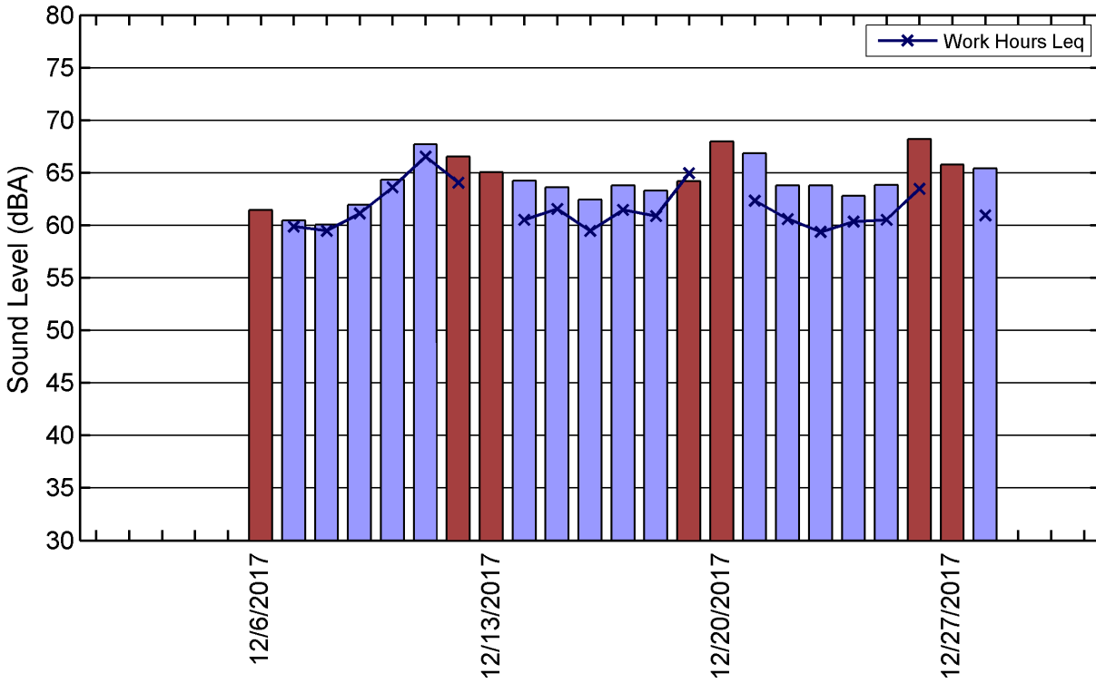
Figure 8: Monitor 5 Ldn and Daytime Leq Results
