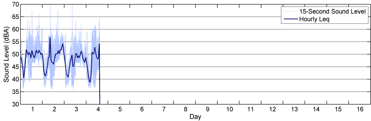
Figure 3: Monitor 5 Hourly Leq Results
