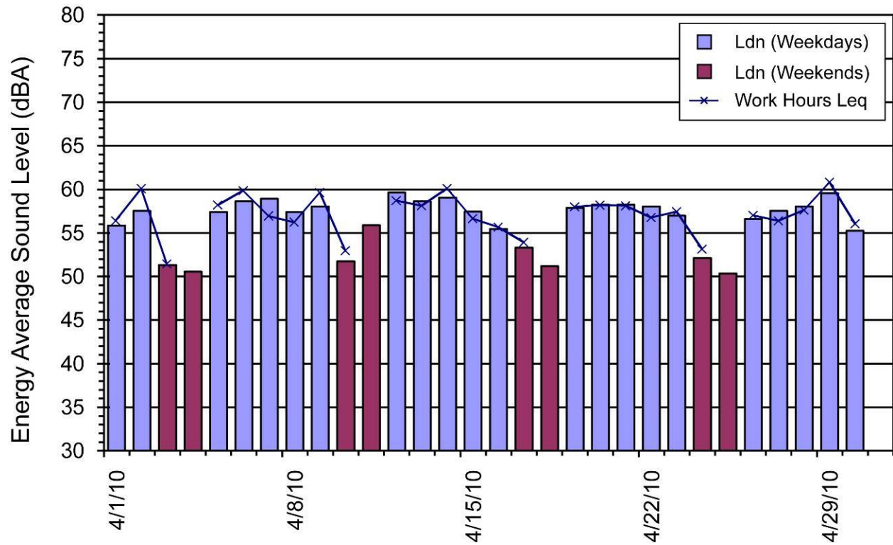
Figure 3: Monitor 1 Ldn and Daytime Leq Results
