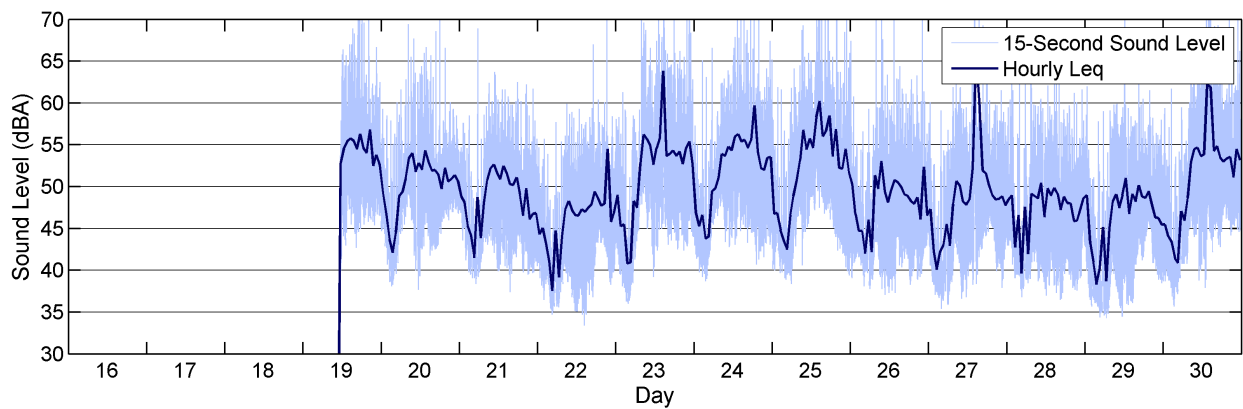
Figure 1: Monitor 8 Hourly Leq Results
