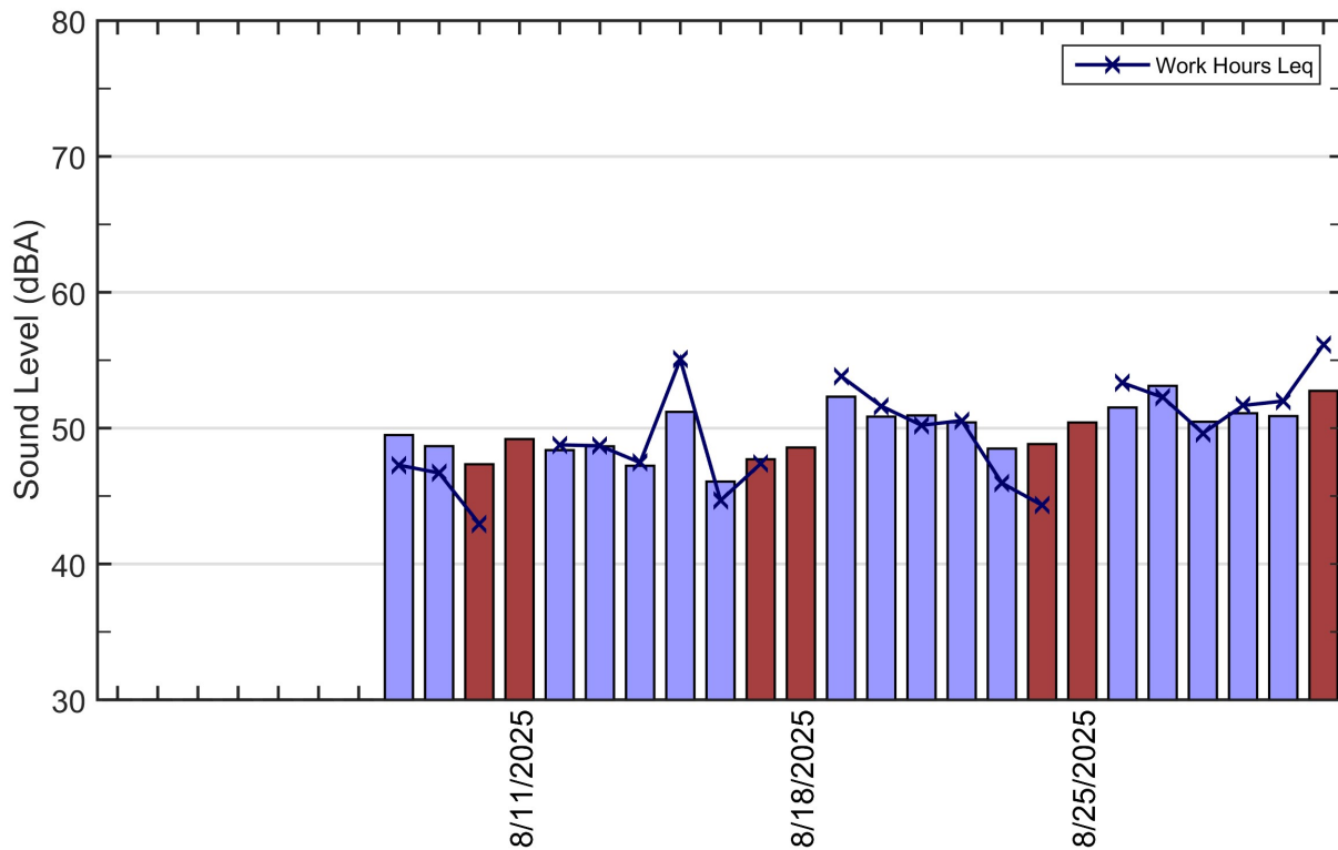
Figure 6: Monitor C Ldn and Daytime Leq Results
