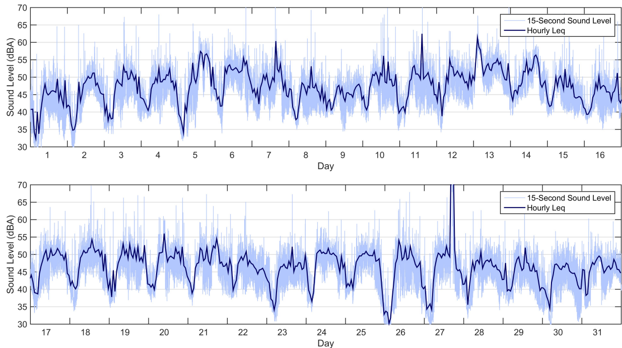
Figure 1: Monitor C Hourly Leq Results
